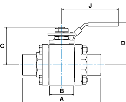
H-510 TUBE SOCKET WELD STANDARD CONFIGURATION DIMENSIONS
