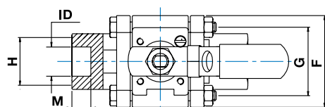
H-510 PIPE SOCKET WELD STANDARD CONFIGURATION DIMENSIONS
