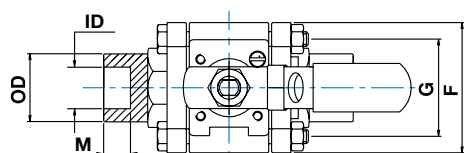
H-510 TUBE SOCKET WELD STANDARD CONFIGURATION DIMENSIONS
