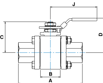
H-510 PIPE SOCKET WELD STANDARD CONFIGURATION DIMENSIONS
