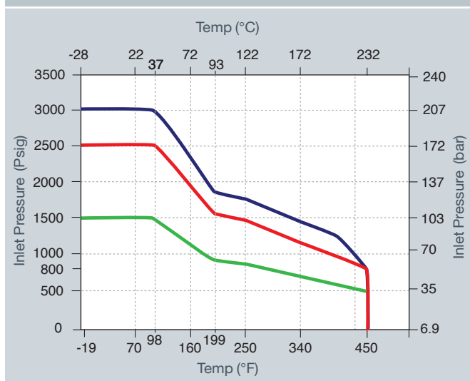
PEEK SEATS
