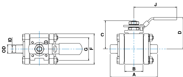
H-580 PIPE BUTTWELD STANDARD CONFIGURATION DIMENSIONS
